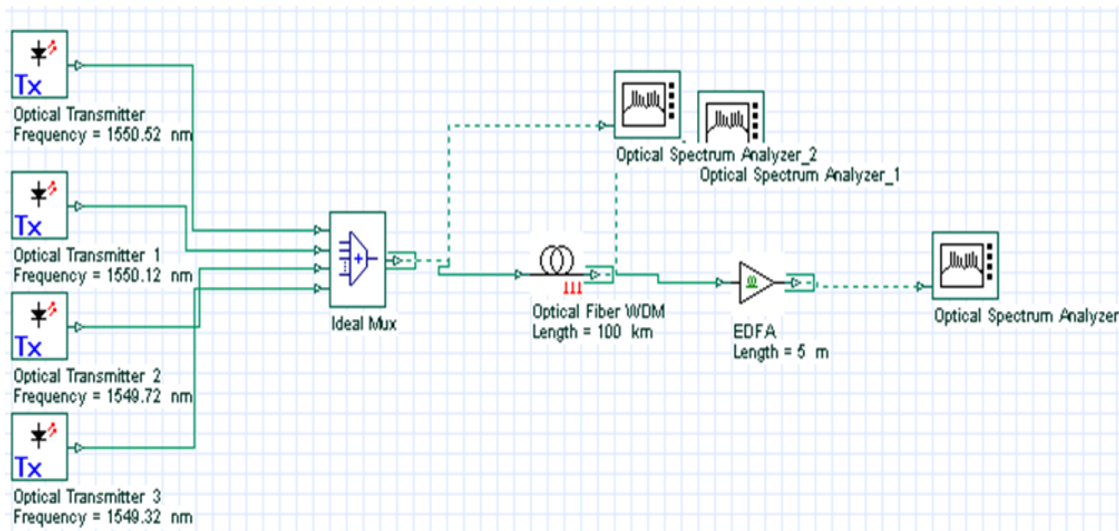
Figure 4: FWM simulation Setup The power measured at the fiber input and output are presented in Table 3.
