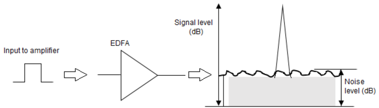
Figure 1: Single stage amplifier and noise associated with the signal [7]
