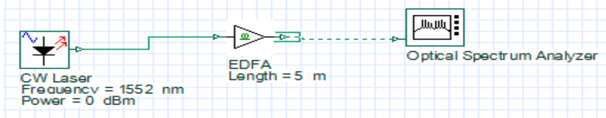
Figure 2: EDFA simulation setup
