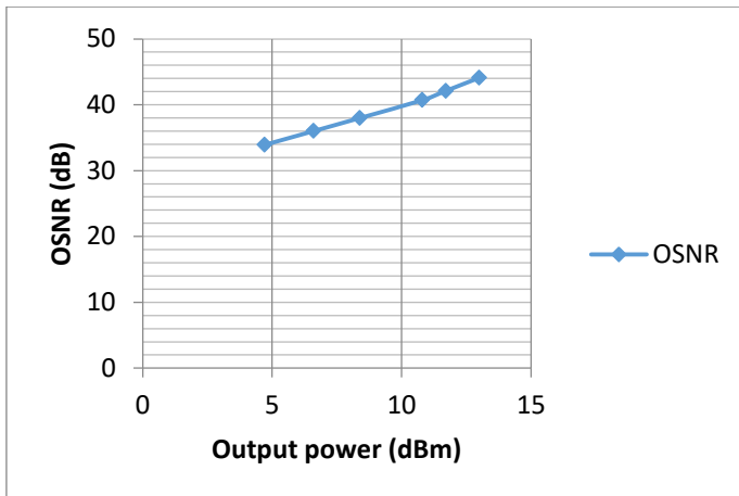
Figure 5: Plot of OSNR against Output Power
