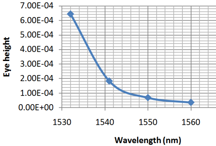
Figure 6: Eye Height against Wavelength
