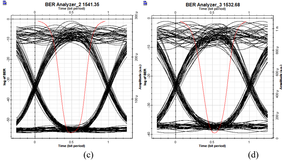
Figure 7: Eye diagrams of the WDM network
