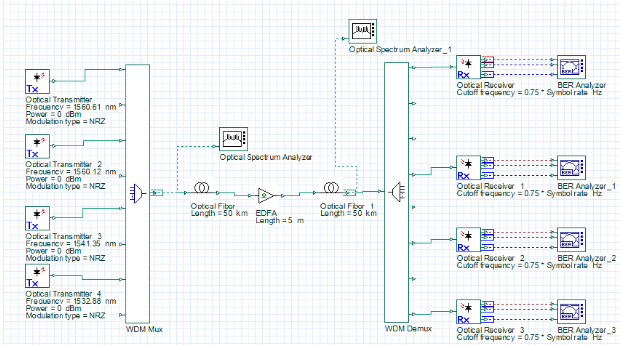
Figure 3: Amplified WDM simulation setup The results are as presented in Section 3.0.
