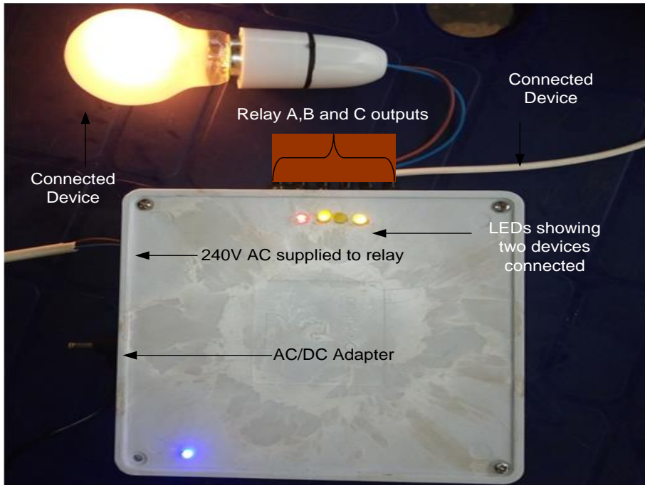
Fig 4.3 the Receiver module connected to home appliances
