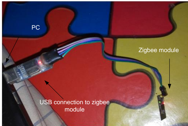
Fig 4.1 Transmitter module connected to a PC
